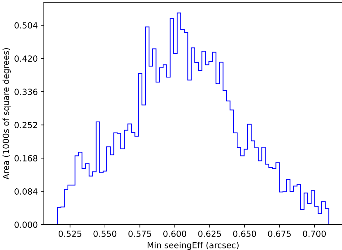
too_elab_heavy_r64_d3_gz_v3.4_10yrs WFD i band: Min seeingEff
