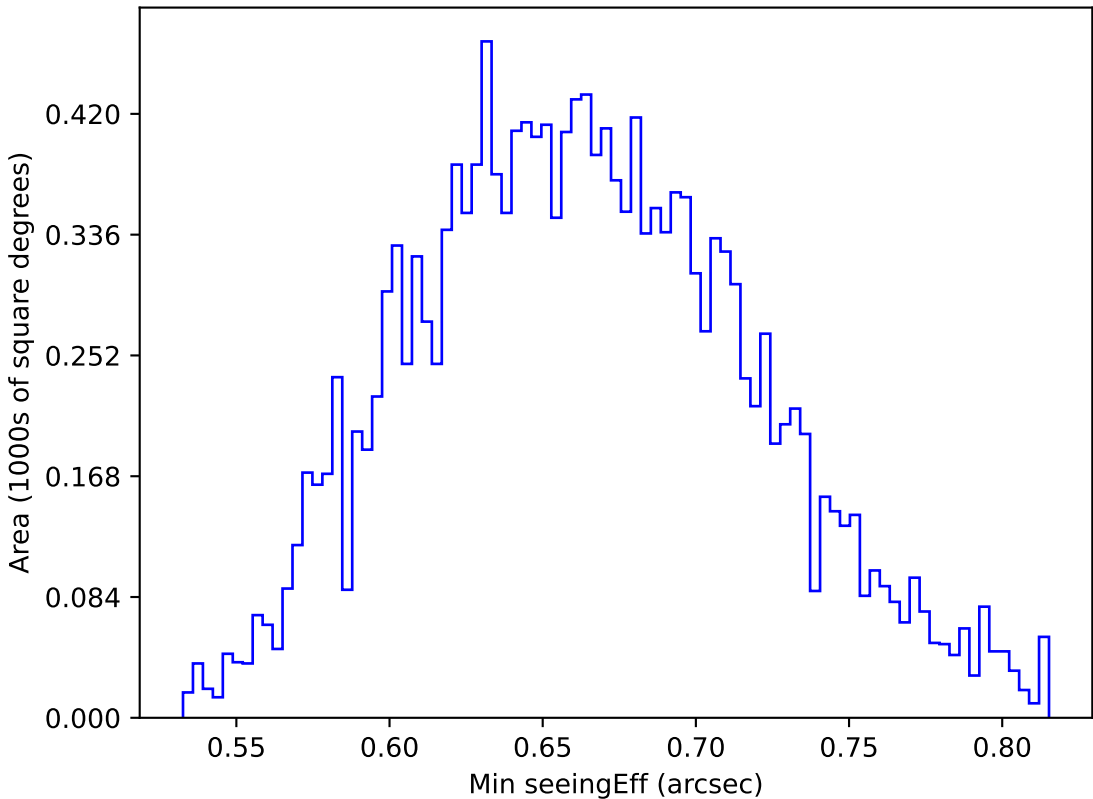
too_elab_heavy_r64_d3_gz_v3.4_10yrs WFD g band: Min seeingEff
