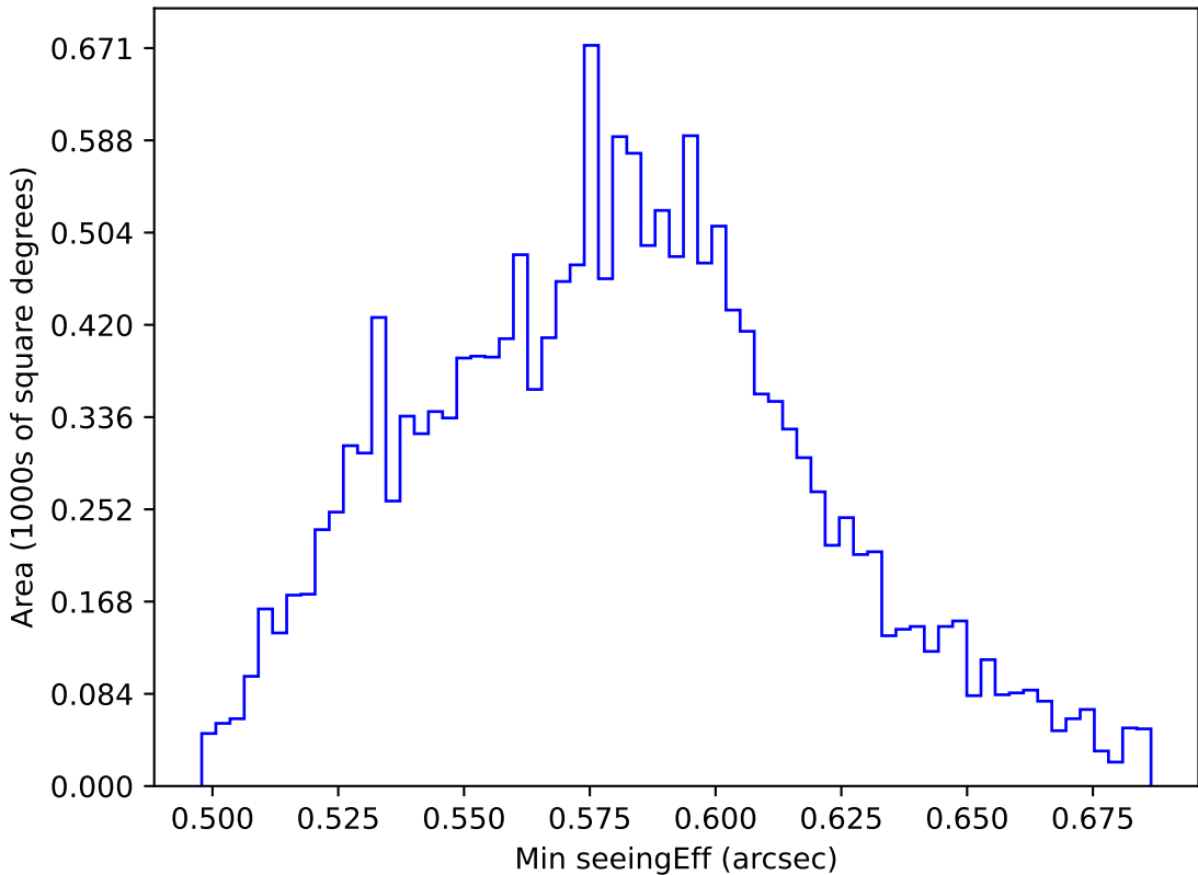
too_elab_heavy_r64_d3_gz_v3.4_10yrs WFD all bands: Min seeingEff
