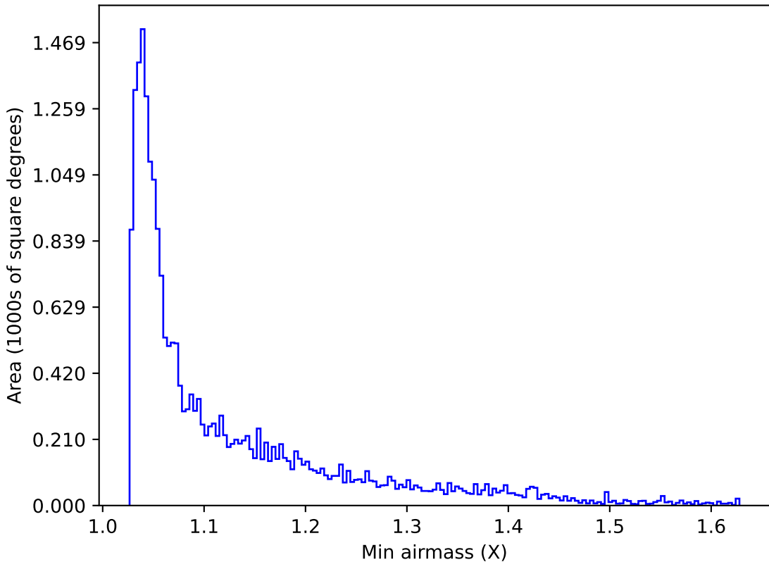
too_elab_heavy_r64_d3_gz_v3.4_10yrs Yr 1 y band: Min airmass
