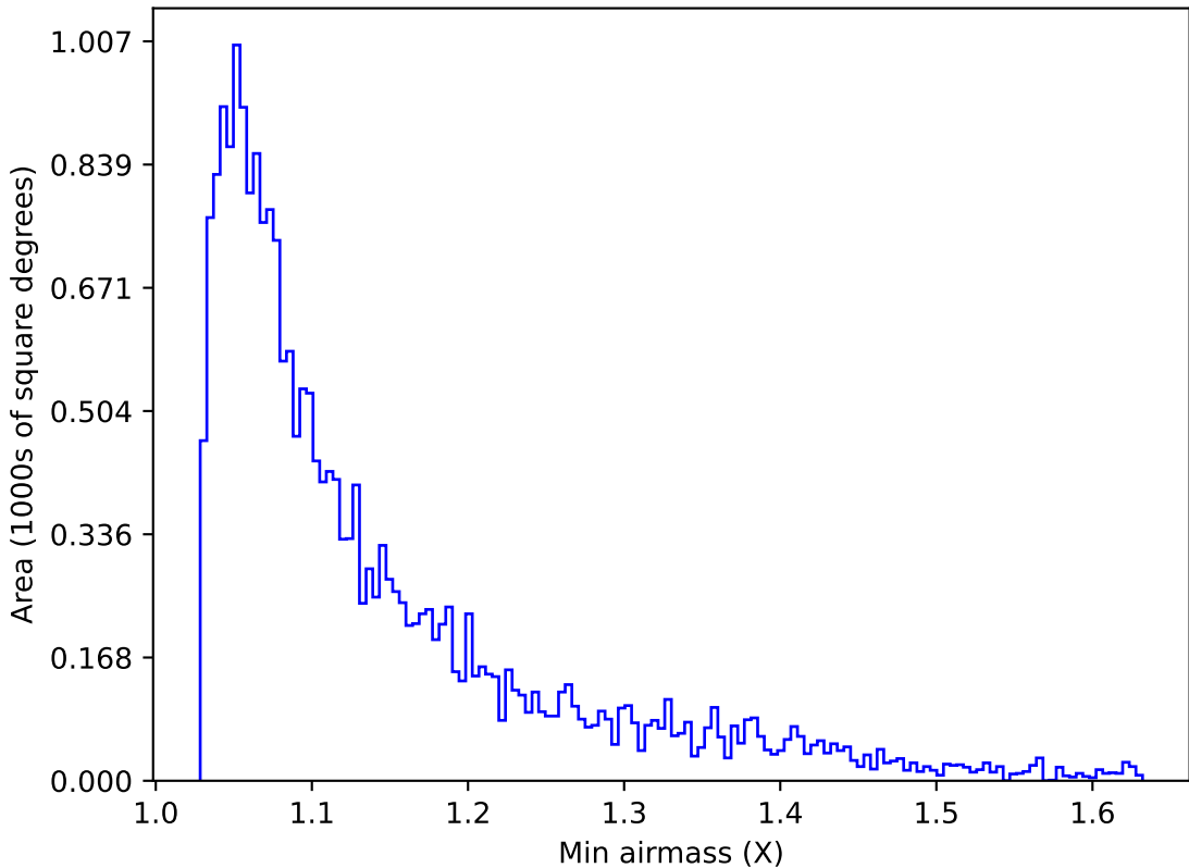
too_elab_heavy_r64_d3_gz_v3.4_10yrs Yr 1 u band: Min airmass
