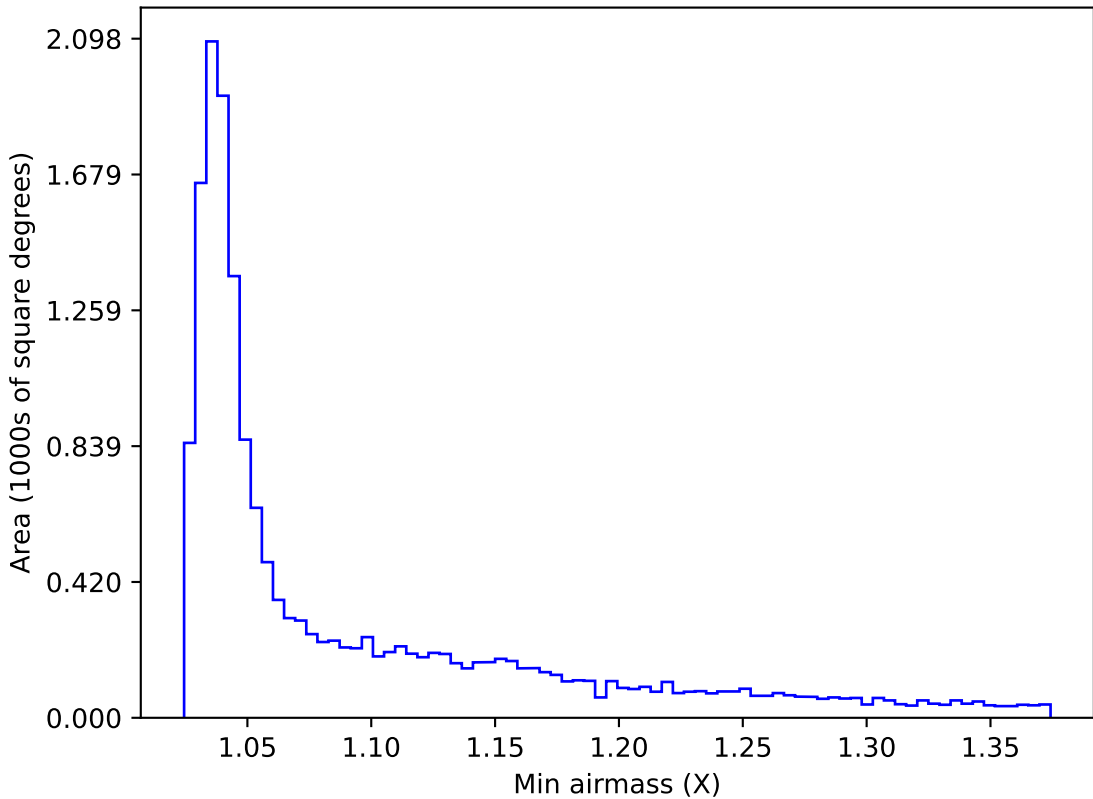
too_elab_heavy_r64_d3_gz_v3.4_10yrs WFD u band: Min airmass
