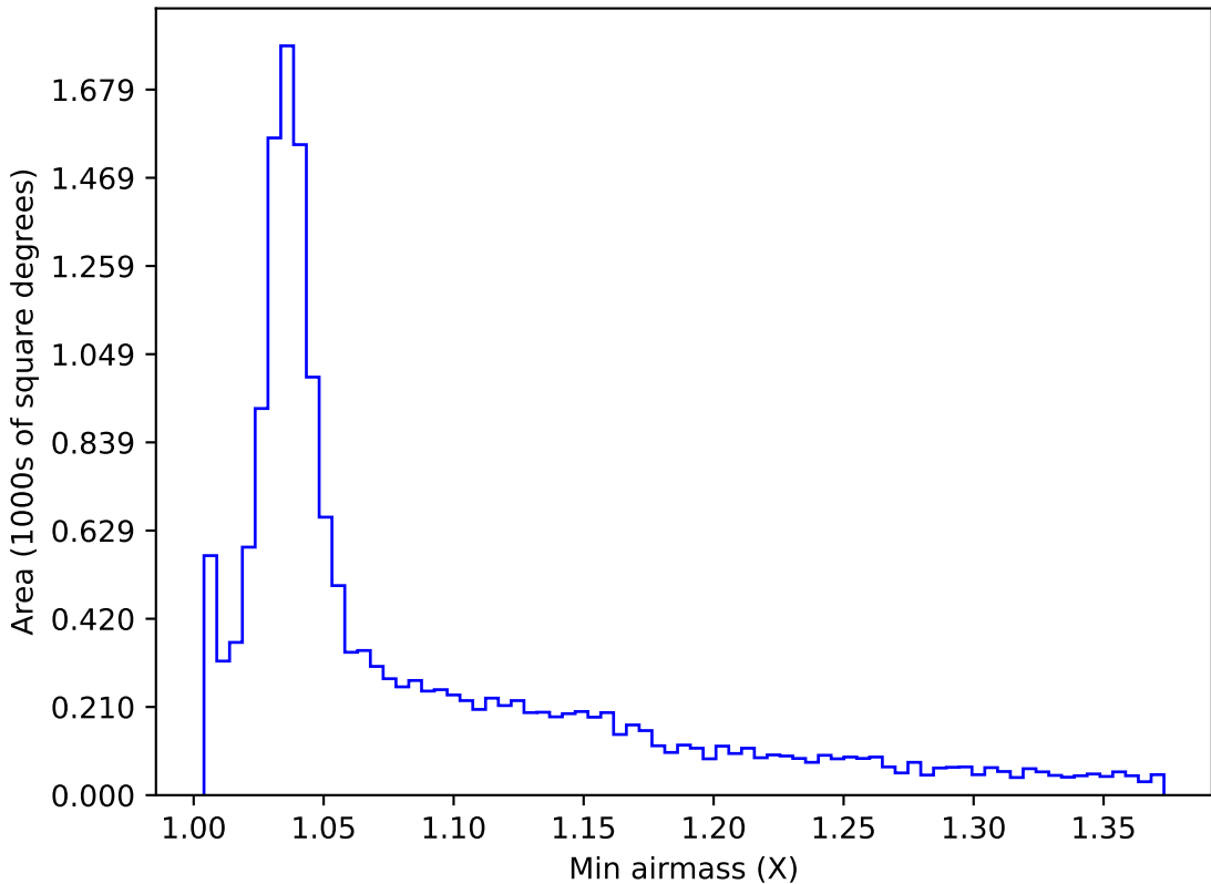
too_elab_heavy_r64_d3_gz_v3.4_10yrs WFD g band: Min airmass
