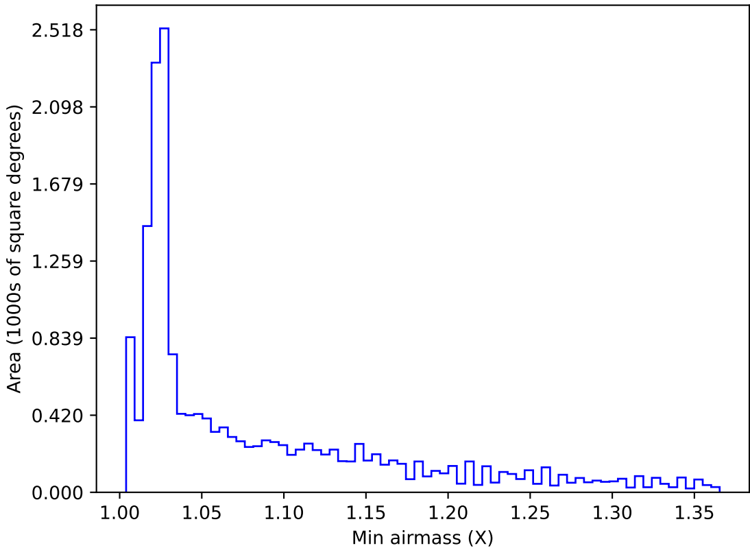
too_elab_heavy_r64_d3_gz_v3.4_10yrs WFD all bands: Min airmass
