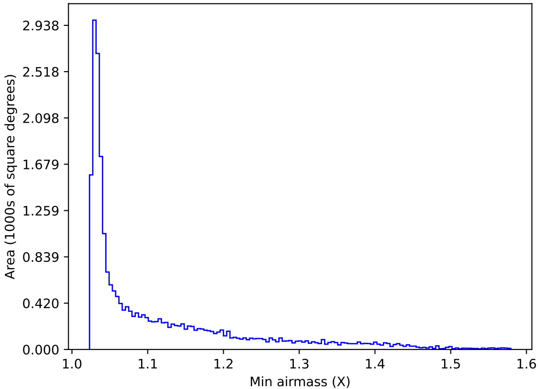
too_elab_heavy_r64_d3_gz_v3.4_10yrs All sky y band: Min airmass
