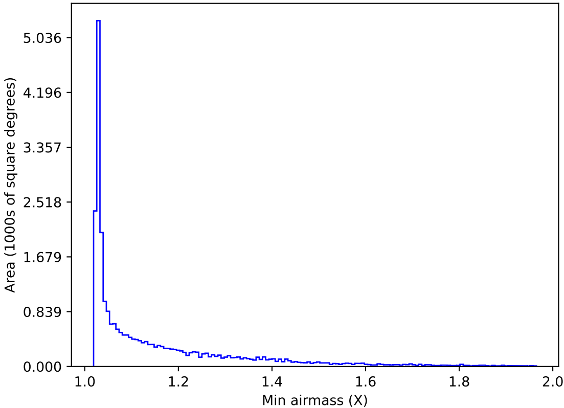
too_elab_heavy_r64_d3_gz_v3.4_10yrs All sky i band: Min airmass
