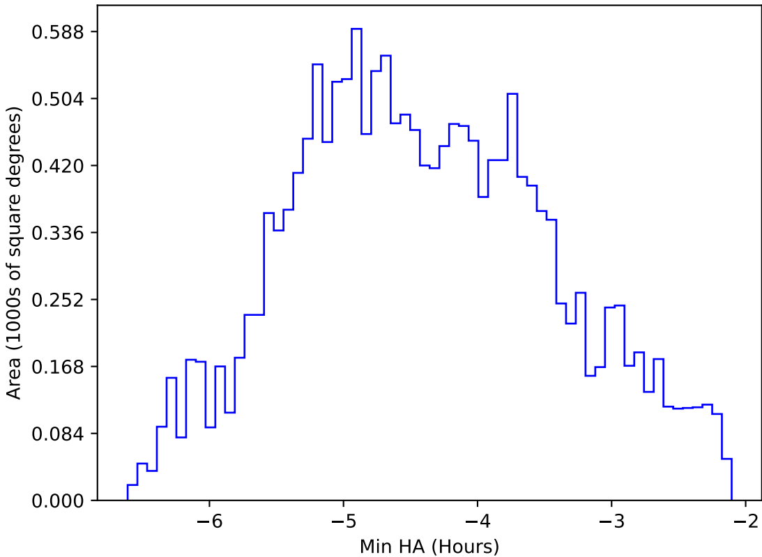
too_elab_heavy_r64_d3_gz_v3.4_10yrs WFD i band: Min HA
