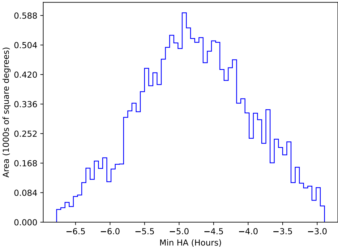
too_elab_heavy_r64_d3_gz_v3.4_10yrs WFD all bands: Min HA
