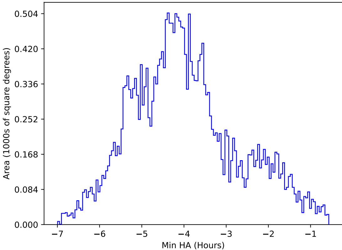
too_elab_heavy_r64_d3_gz_v3.4_10yrs All sky z band: Min HA
