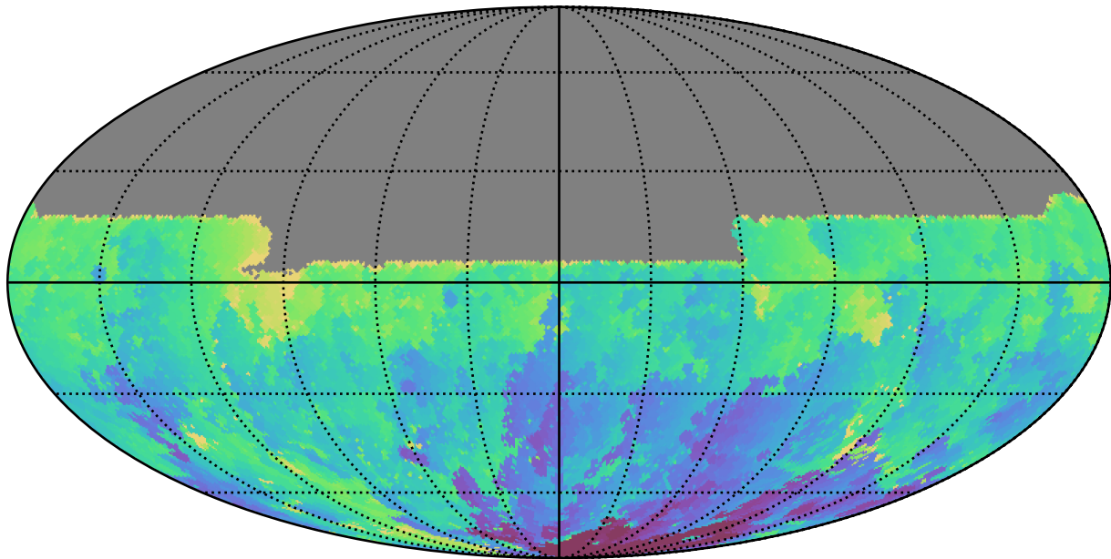
too_elab_heavy_r64_d3_gz_v3.4_10yrs All sky u band: Min HA
