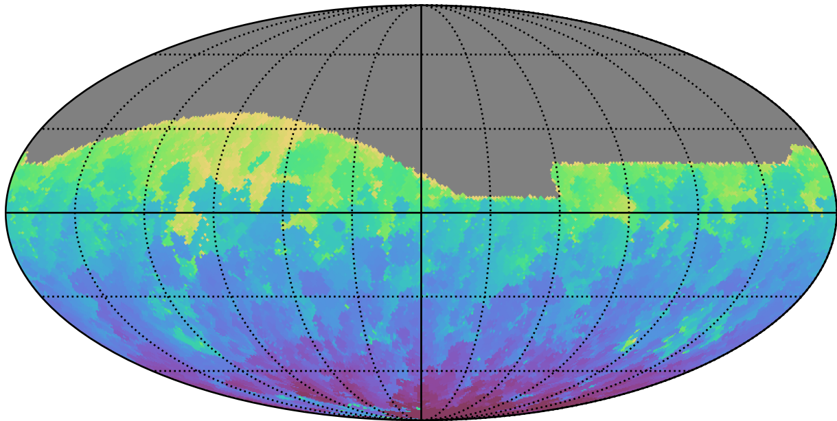
too_elab_heavy_r64_d3_gz_v3.4_10yrs All sky g band: Min HA
