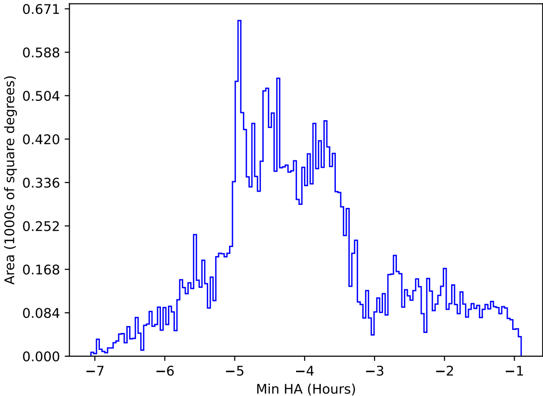
too_elab_heavy_r64_d3_gz_v3.4_10yrs All sky g band: Min HA
