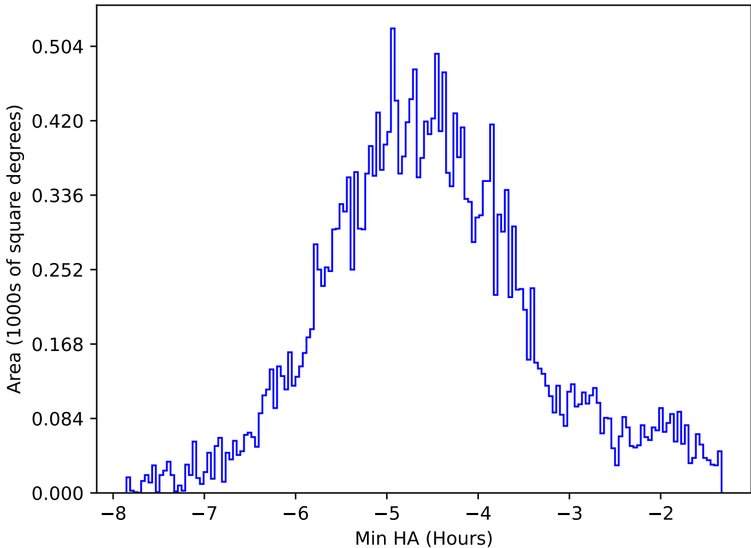
too_elab_heavy_r64_d3_gz_v3.4_10yrs All sky all bands: Min HA
