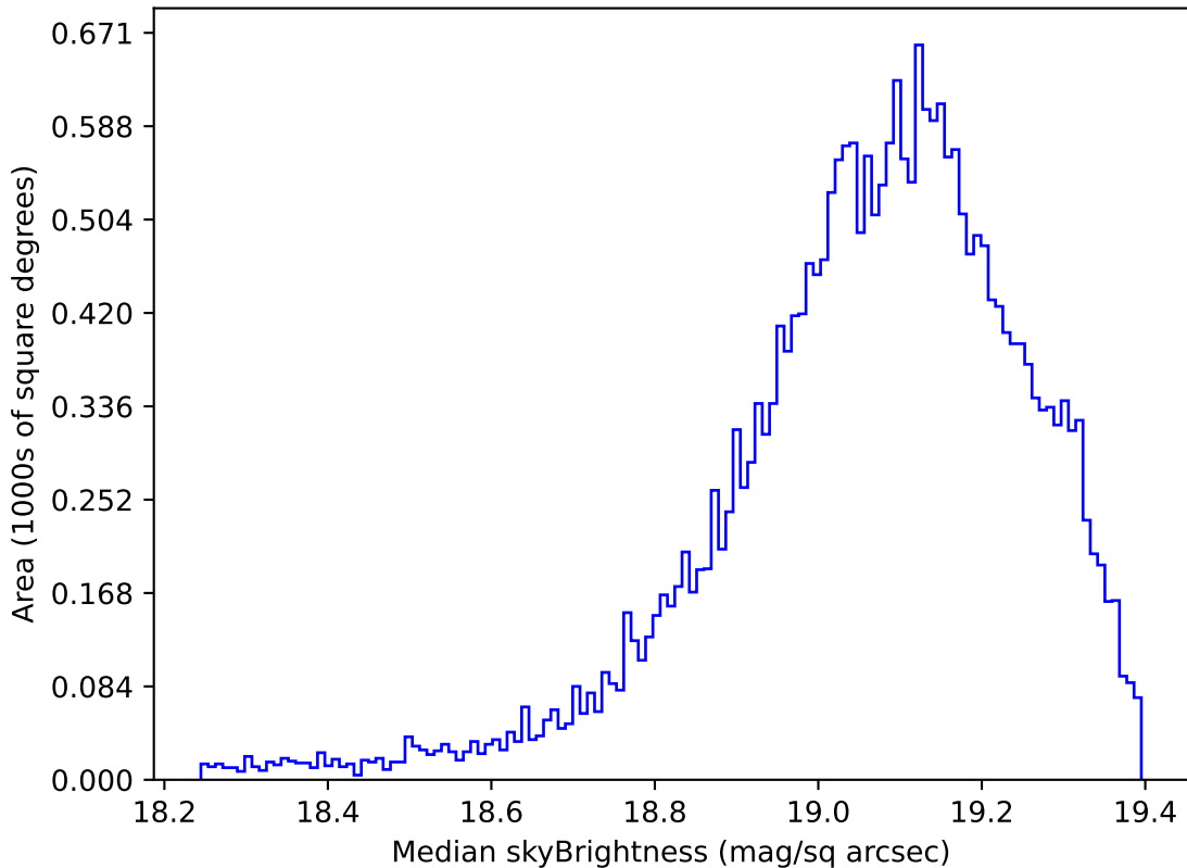
too_elab_heavy_r64_d3_gz_v3.4_10yrs Yr 1 z band: Median skyBrightness
