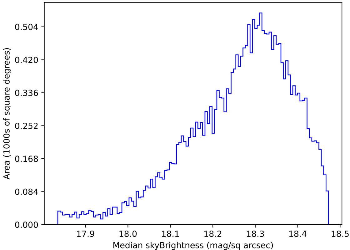
too_elab_heavy_r64_d3_gz_v3.4_10yrs Yr 1 y band: Median skyBrightness
