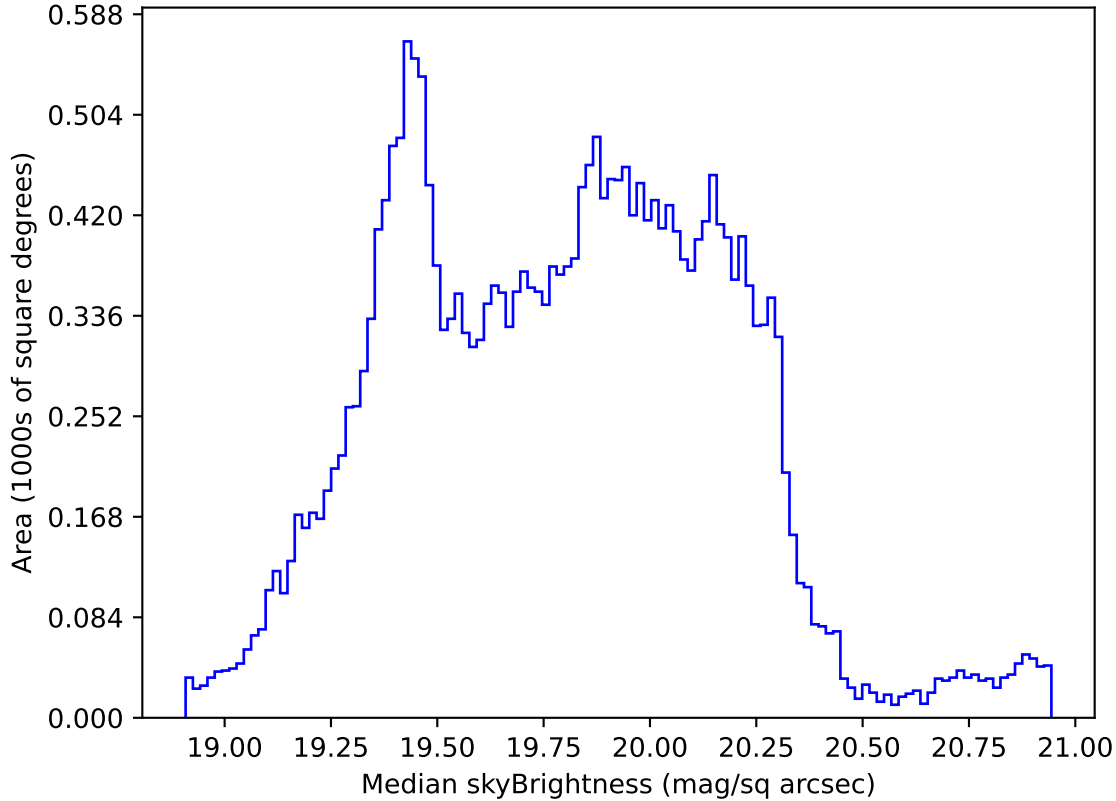
too_elab_heavy_r64_d3_gz_v3.4_10yrs Yr 1 all bands: Median skyBrightness
