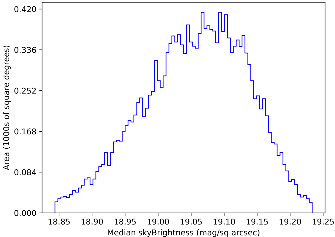
too_elab_heavy_r64_d3_gz_v3.4_10yrs WFD z band: Median skyBrightness
