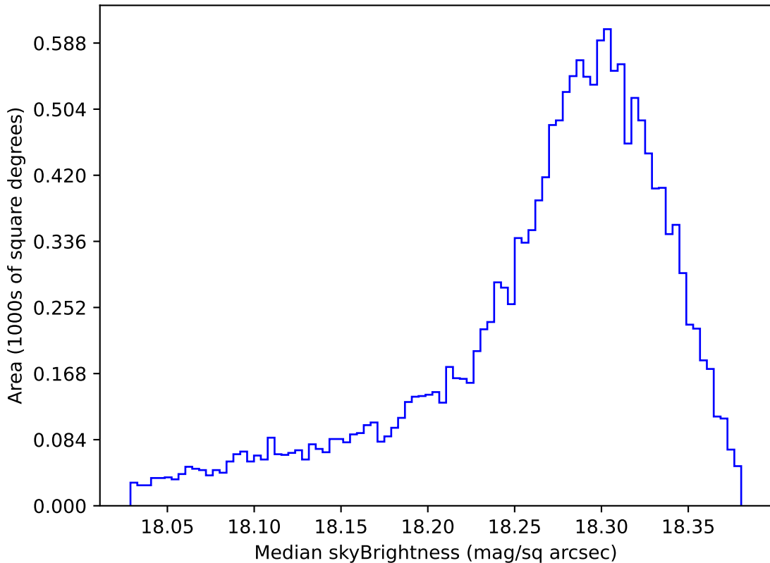
too_elab_heavy_r64_d3_gz_v3.4_10yrs WFD y band: Median skyBrightness
