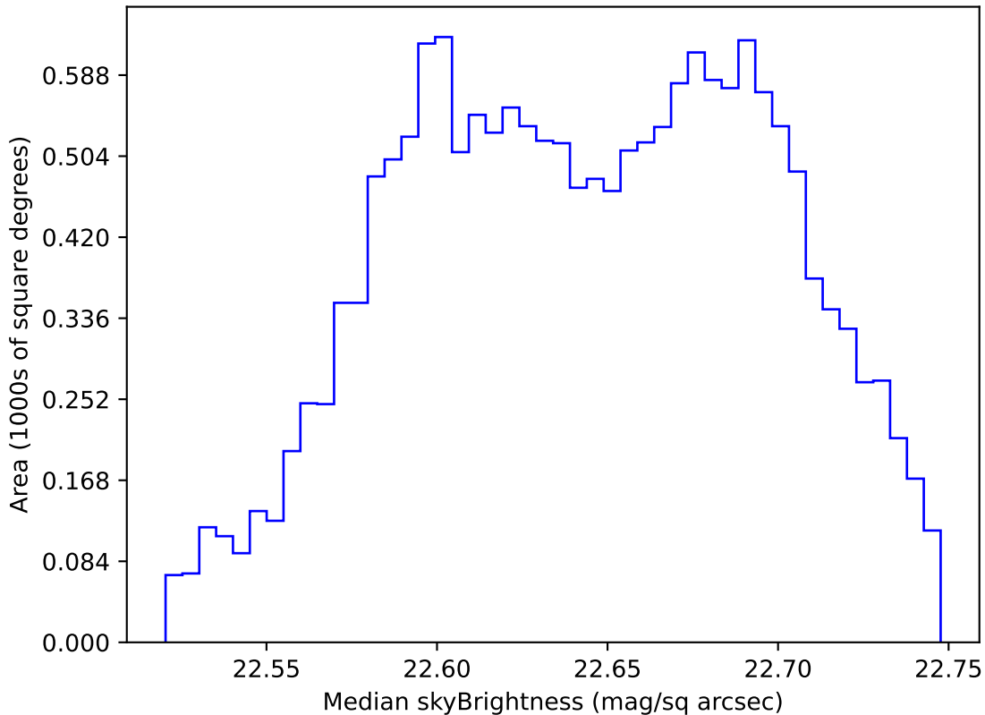
too_elab_heavy_r64_d3_gz_v3.4_10yrs WFD u band: Median skyBrightness
