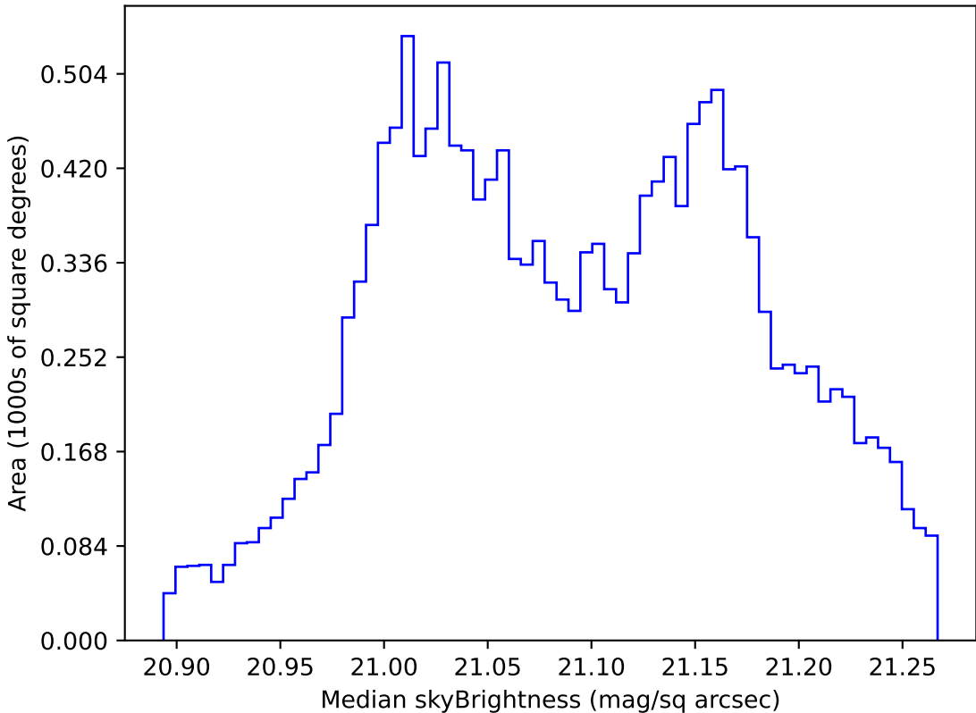
too_elab_heavy_r64_d3_gz_v3.4_10yrs WFD r band: Median skyBrightness
