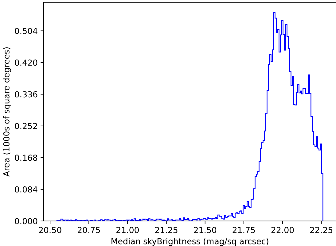
too_elab_heavy_r64_d3_gz_v3.4_10yrs WFD g band: Median skyBrightness
