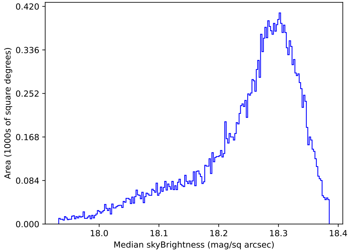
too_elab_heavy_r64_d3_gz_v3.4_10yrs All sky y band: Median skyBrightness
