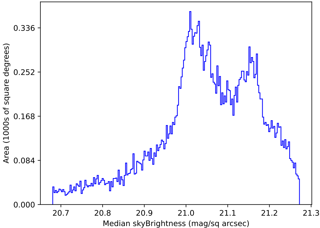
too_elab_heavy_r64_d3_gz_v3.4_10yrs All sky r band: Median skyBrightness
