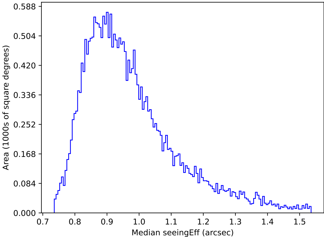
too_elab_heavy_r64_d3_gz_v3.4_10yrs Yr 1 r band: Median seeingEff
