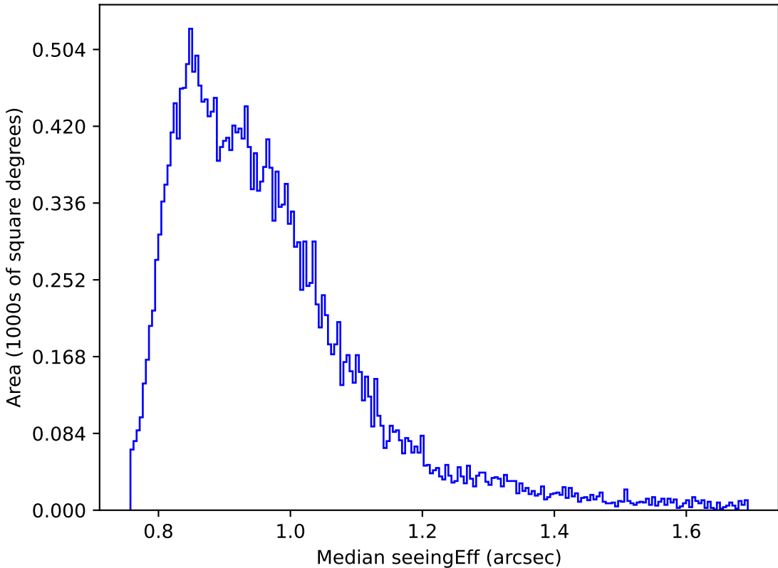
too_elab_heavy_r64_d3_gz_v3.4_10yrs Yr 1 i band: Median seeingEff
