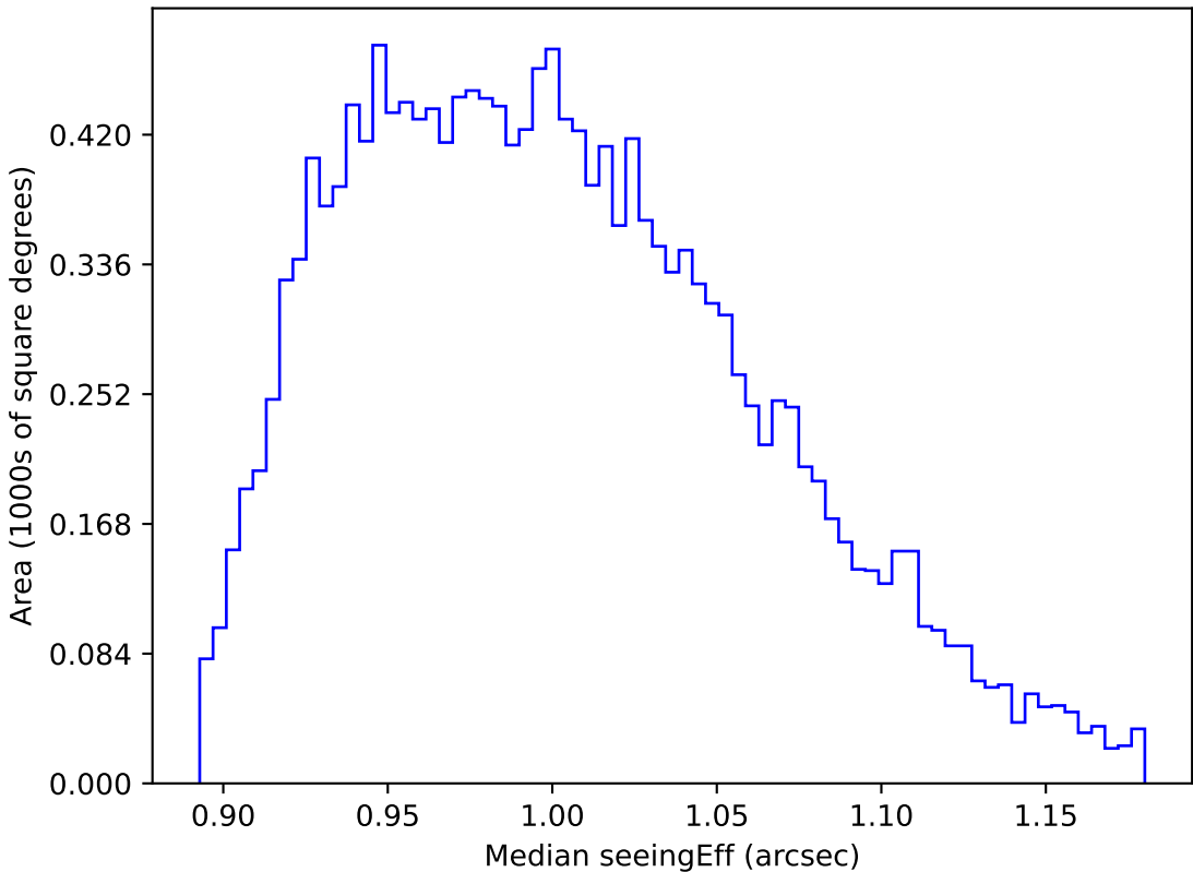
too_elab_heavy_r64_d3_gz_v3.4_10yrs WFD y band: Median seeingEff
