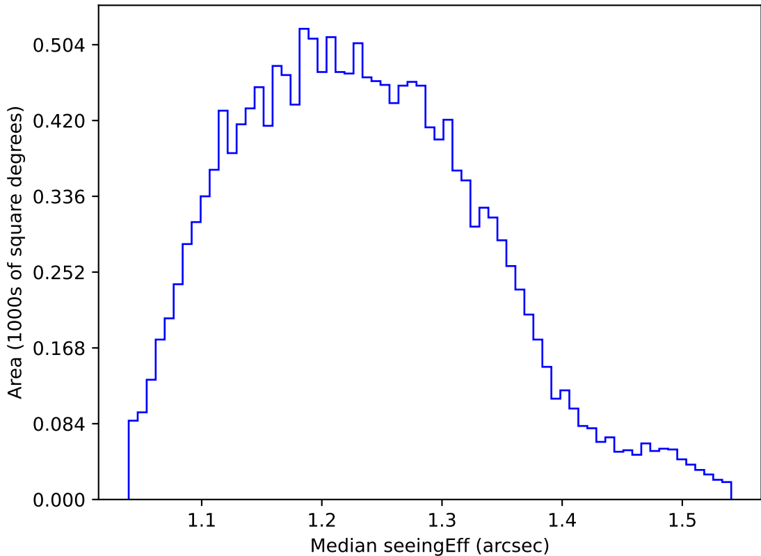
too_elab_heavy_r64_d3_gz_v3.4_10yrs WFD u band: Median seeingEff
