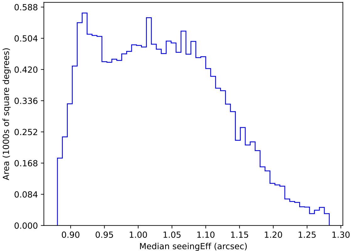
too_elab_heavy_r64_d3_gz_v3.4_10yrs WFD r band: Median seeingEff
