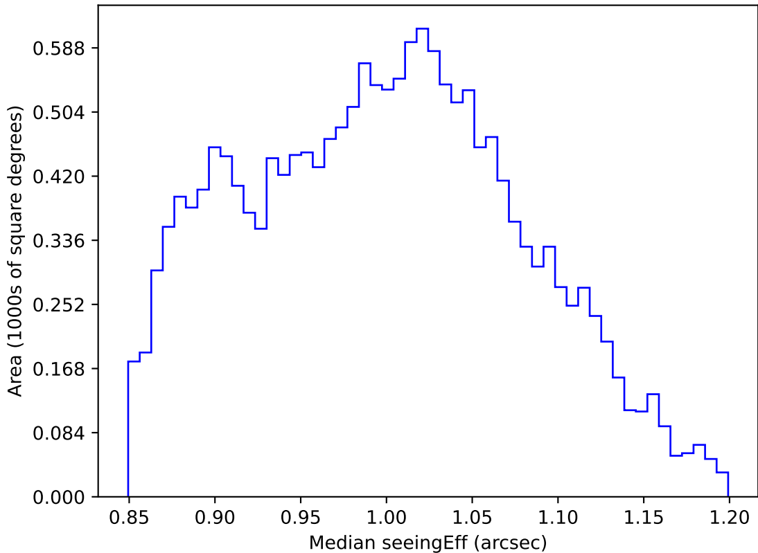
too_elab_heavy_r64_d3_gz_v3.4_10yrs WFD i band: Median seeingEff
