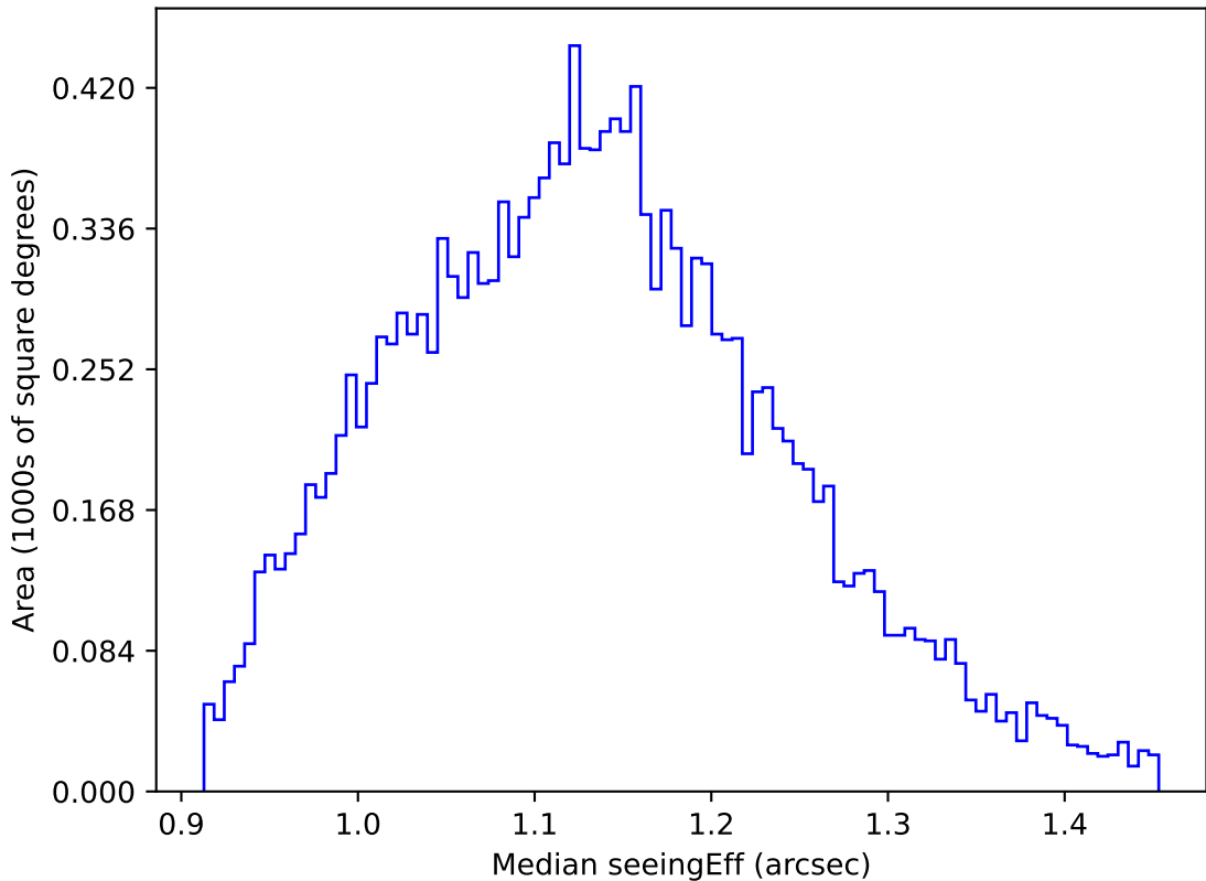
too_elab_heavy_r64_d3_gz_v3.4_10yrs WFD g band: Median seeingEff
