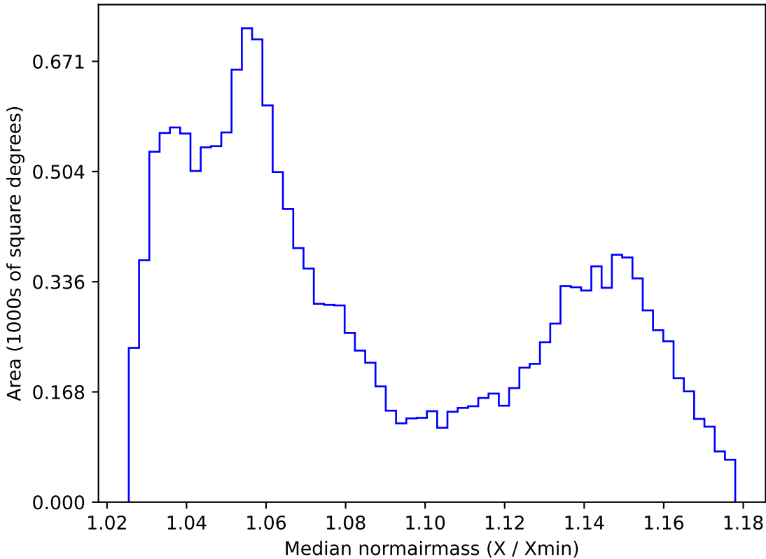
too_elab_heavy_r64_d3_gz_v3.4_10yrs WFD all bands: Median normairmass
