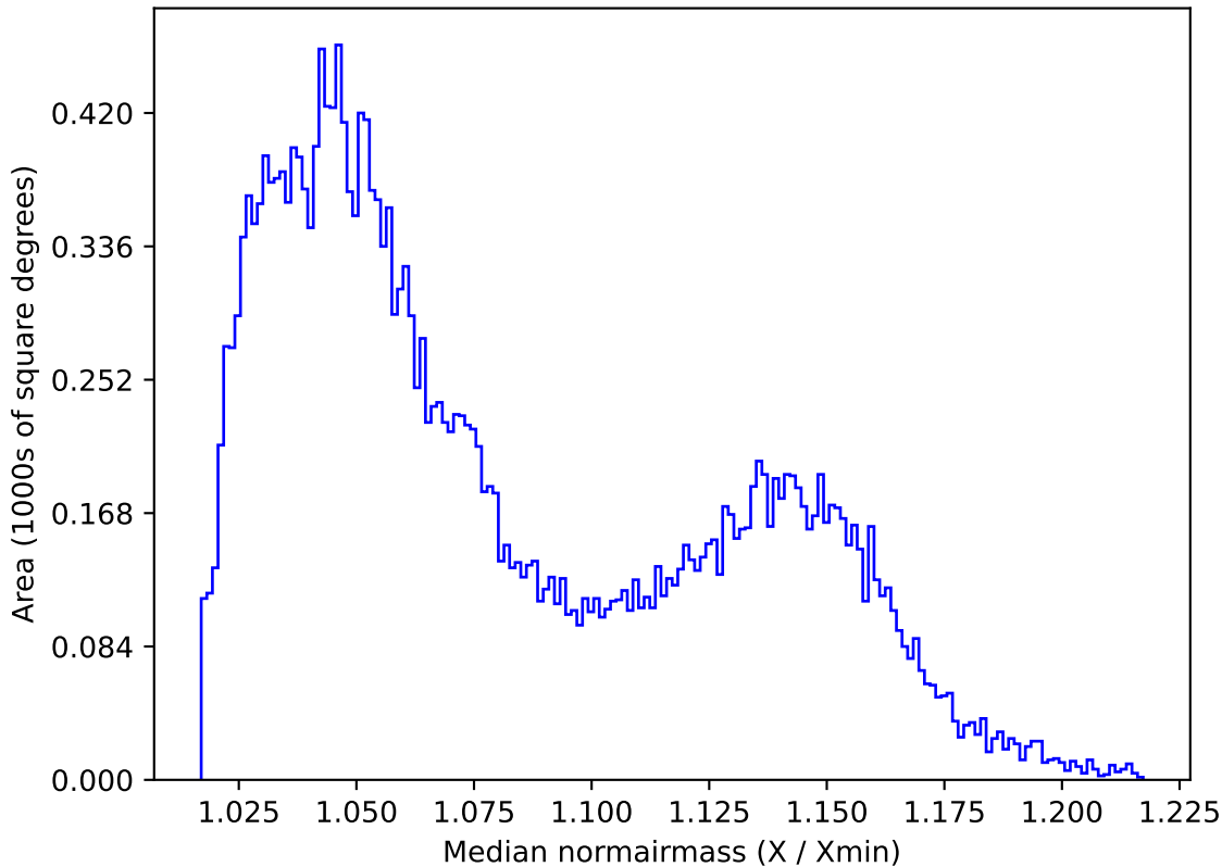
too_elab_heavy_r64_d3_gz_v3.4_10yrs All sky i band: Median normairmass
