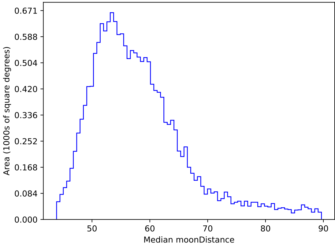
too_elab_heavy_r64_d3_gz_v3.4_10yrs WFD y band: Median moonDistance
