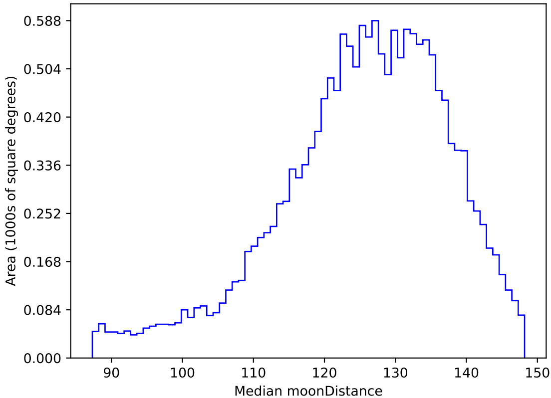
too_elab_heavy_r64_d3_gz_v3.4_10yrs WFD u band: Median moonDistance
