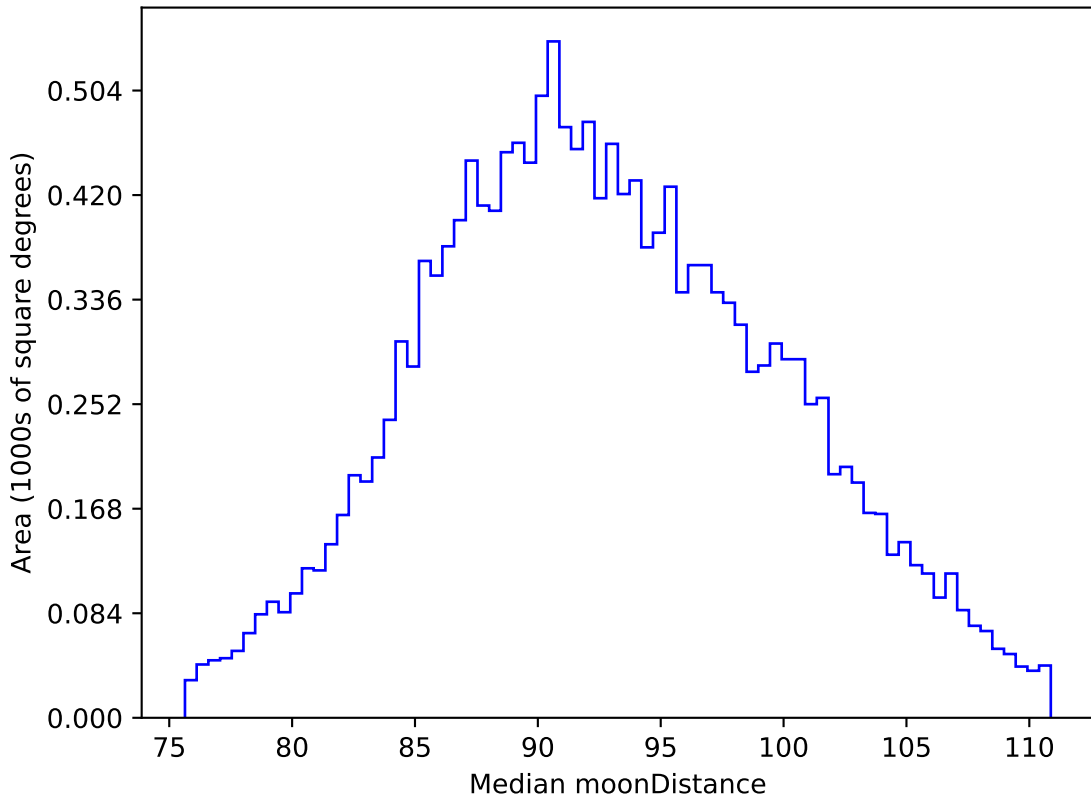
too_elab_heavy_r64_d3_gz_v3.4_10yrs WFD i band: Median moonDistance
