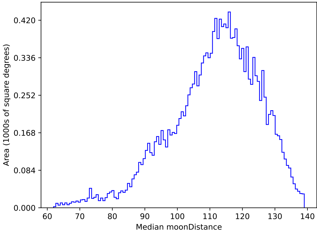
too_elab_heavy_r64_d3_gz_v3.4_10yrs WFD g band: Median moonDistance
