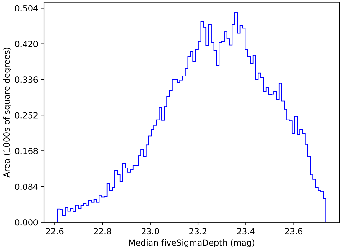
too_elab_heavy_r64_d3_gz_v3.4_10yrs Yr 1 u band: Median fiveSigmaDepth
