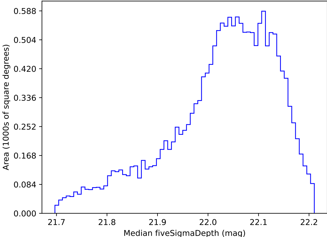
too_elab_heavy_r64_d3_gz_v3.4_10yrs WFD y band: Median fiveSigmaDepth
