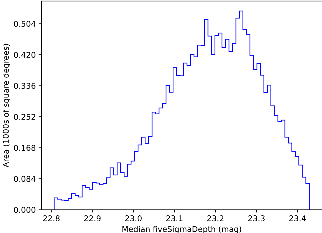
too_elab_heavy_r64_d3_gz_v3.4_10yrs WFD u band: Median fiveSigmaDepth
