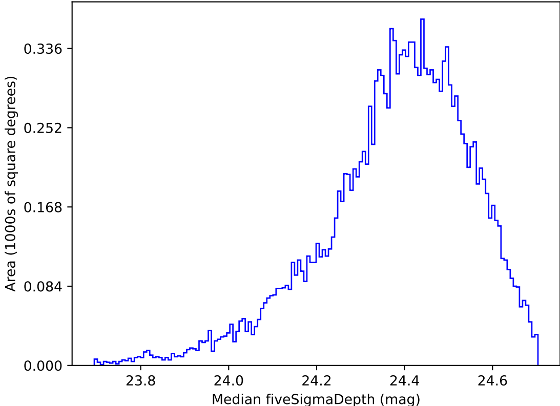
too_elab_heavy_r64_d3_gz_v3.4_10yrs WFD g band: Median fiveSigmaDepth
