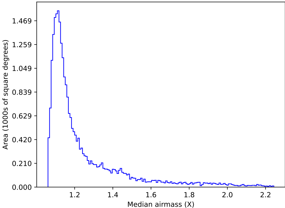
too_elab_heavy_r64_d3_gz_v3.4_10yrs Yr 1 i band: Median airmass
