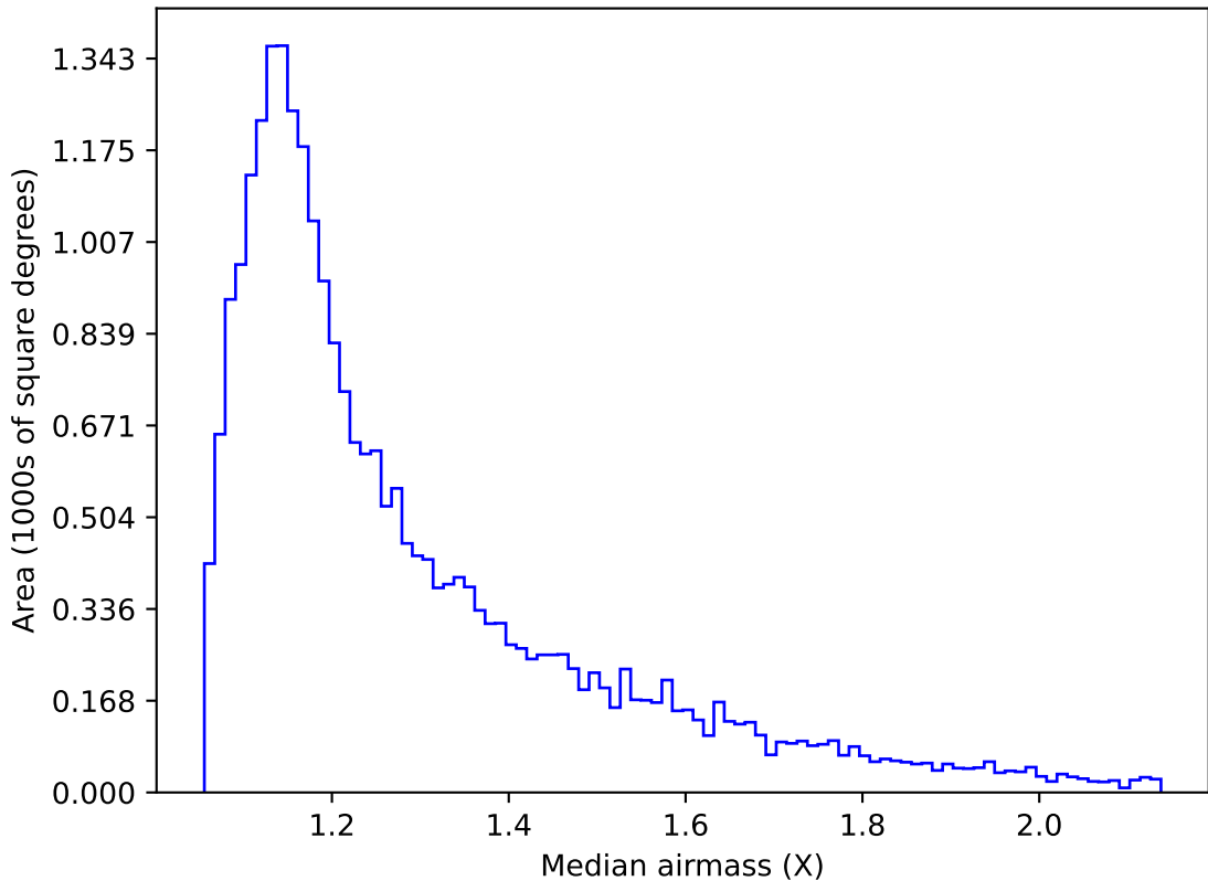
too_elab_heavy_r64_d3_gz_v3.4_10yrs Yr 1 g band: Median airmass
