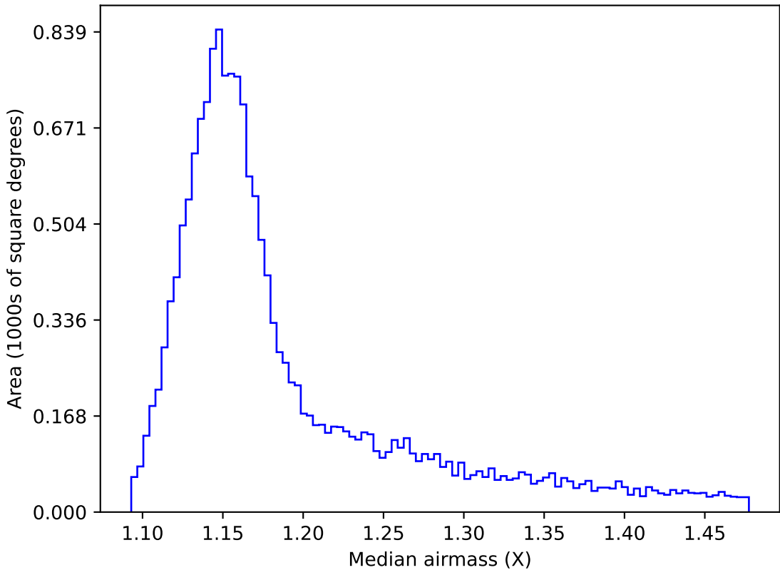
too_elab_heavy_r64_d3_gz_v3.4_10yrs WFD y band: Median airmass
