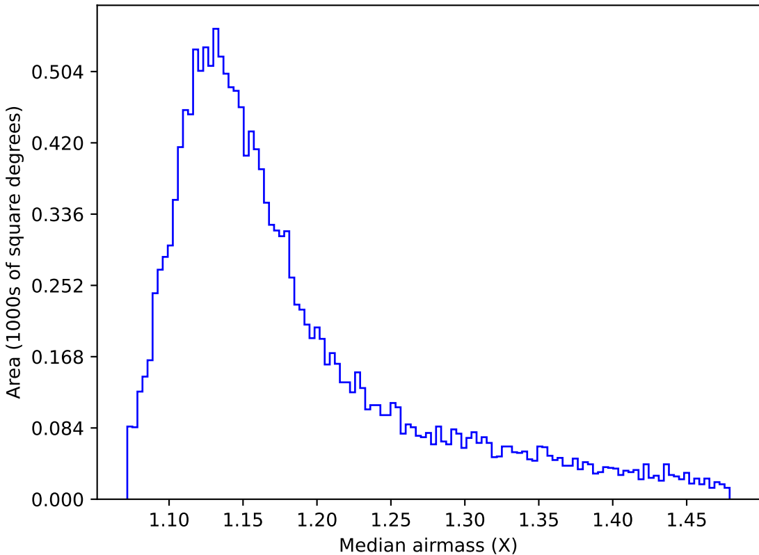
too_elab_heavy_r64_d3_gz_v3.4_10yrs WFD u band: Median airmass
