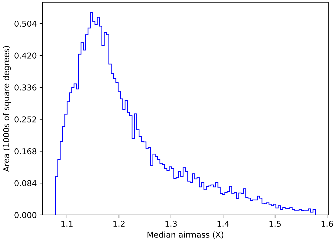
too_elab_heavy_r64_d3_gz_v3.4_10yrs WFD g band: Median airmass
