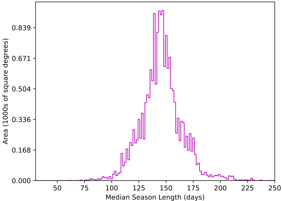
too_elab_heavy_r64_d3_gz_v3.4_10yrs WFD z band: Median Season Length
